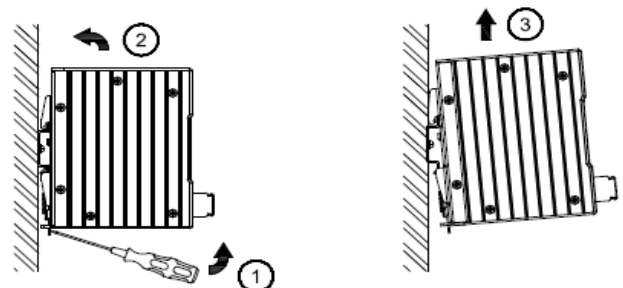
Fig. 2.2 Dismounting
