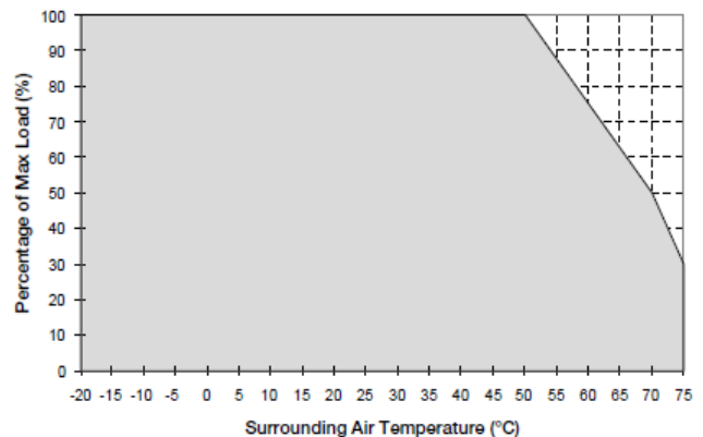
Fig. 1.2 De-rating for Horizontal Mounting Orientation > 50°C de-rate power by 2.5% / °C, > 70°C de-rate power by 4% / °C
